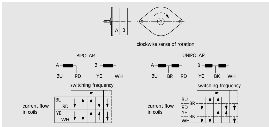
Connections RDM 36/12
