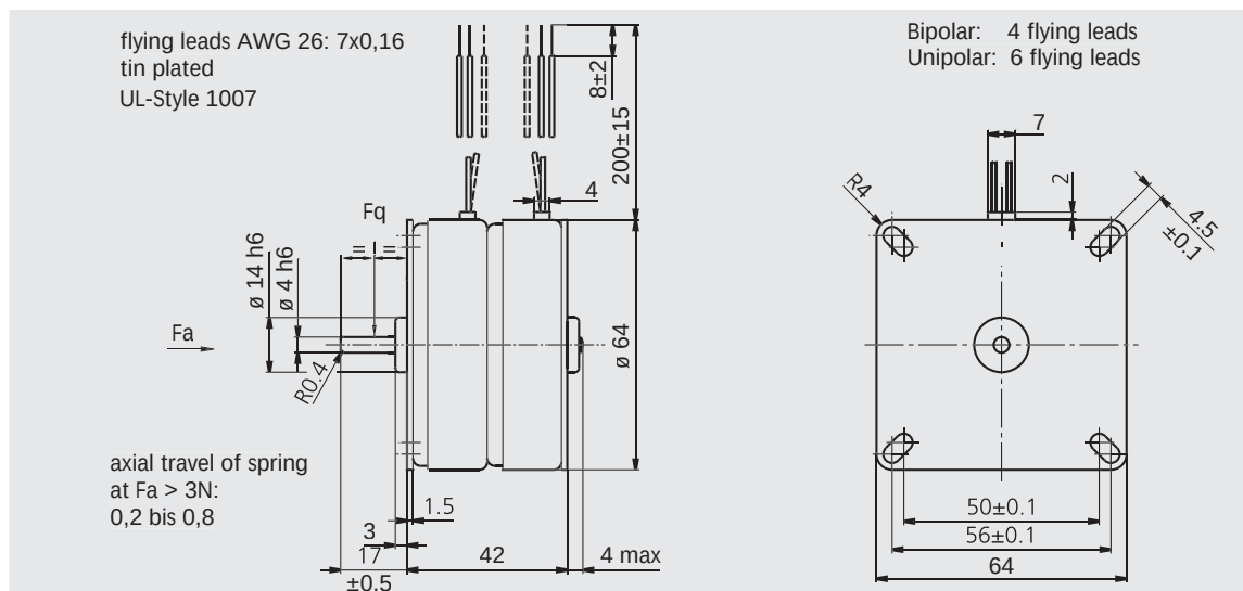
Scale drawing RDM 63/12
