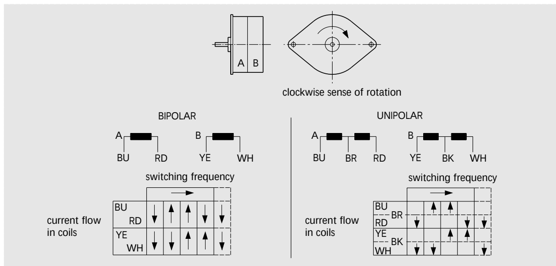
Connections RDM 36/6
